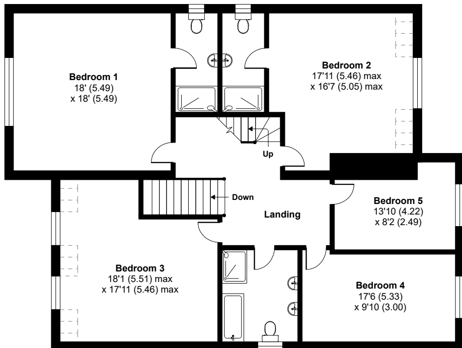
FIRST FLOOR
